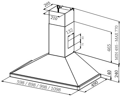
CLASSIC/FALCON AFZUIGKAP/ Plus
